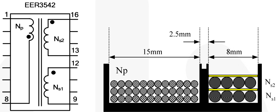
Figure 30. Transformer Construction
