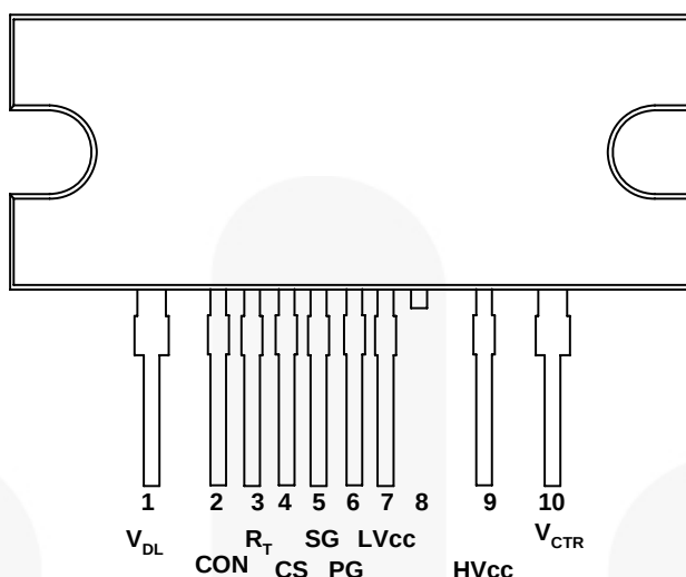
Figure 3. Package Diagram
