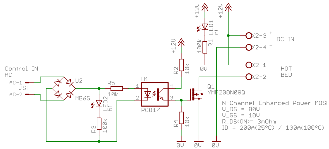
3D Printer MOSFED Circuit for HOT BED
