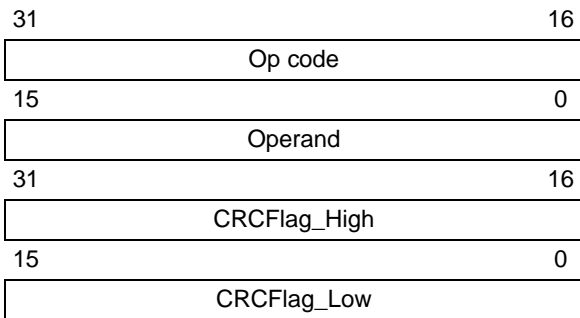
FIGURE 16-26: CHANGE_CFG COMMAND
