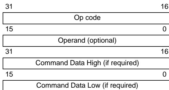
FIGURE 16-1: COMMAND FORMAT
