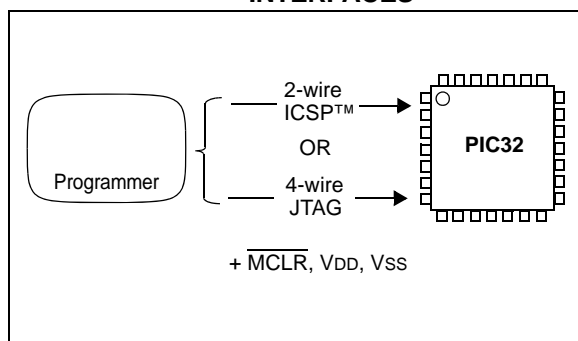
FIGURE 4-1: PROGRAMMING INTERFACES
