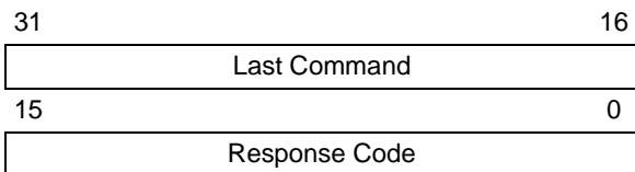
FIGURE 16-27: CHANGE_CFG RESPONSE
